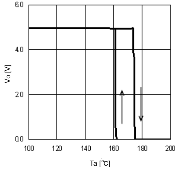
Fig.28 TSD ( I_o=0mA )
