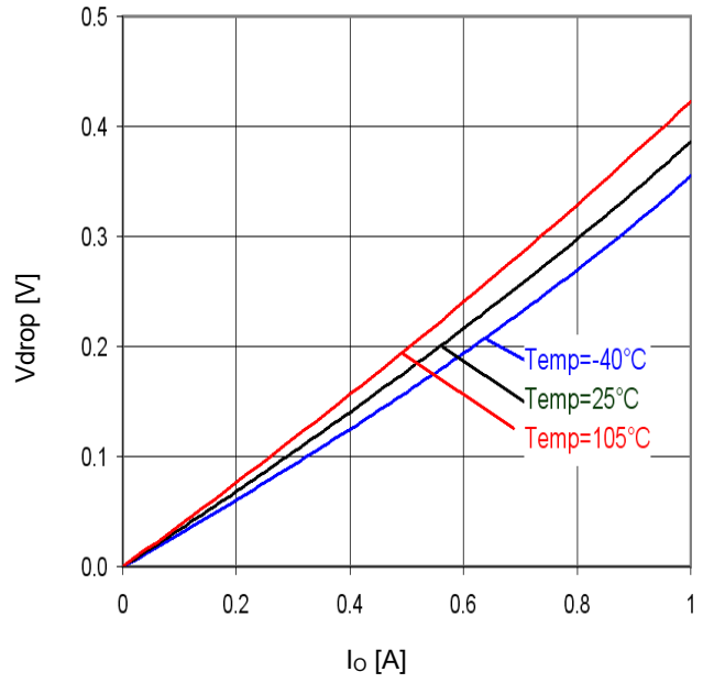
Fig.36 Minimum dropout Voltage 2 (Vcc=4V, Ta=25°C)
