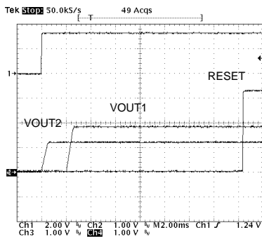
Fig.18 Soft start waveform (Io1=0mA,Io2=0mA,RESET)
