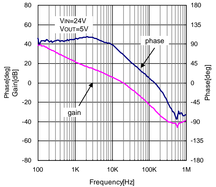
Figure 38. Loop Response (VIN=24V, VOUT=5V, IOUT=2.5A, COUT=Ceramic22μF × 2)
