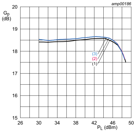
V_{DS} = 28\text{ V}; I_{Dq} = 864\text{ mA}. (1) f = 2112.5\text{ MHz} (2) f = 2140\text{ MHz} (3) f = 2167.5\text{ MHz}
