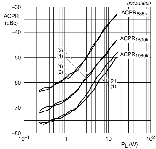
V_{DS} = 28\text{ V} ; I_{Dq} = 225\text{ mA} ; f = 3500\text{ MHz} ; single carrier N-CDMA; PAR = 9.7 dB at 0.01 % probability; channel bandwidth = 1.23 MHz; IBW = 30 kHz.
