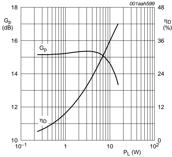
V_{DS} = 28\text{ V} ; I_{Dq} = 225\text{ mA} ; f = 3500\text{ MHz} ; single carrier N-CDMA; PAR = 9.7 dB at 0.01 % probability; channel bandwidth = 1.23 MHz; IBW = 30 kHz.
