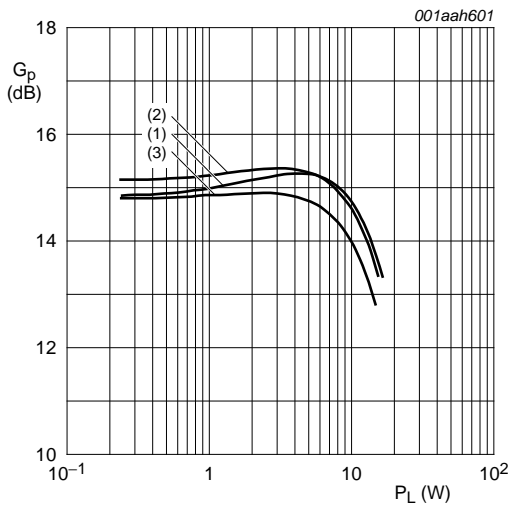
V_{DS} = 28\text{ V} ; I_{Dq} = 225\text{ mA} ; single carrier N-CDMA; PAR = 9.7 dB at 0.01 % probability; channel bandwidth = 1.23 MHz; IBW = 30 kHz.
