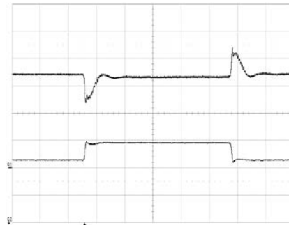
Output voltage response to load current step- change (15-45 A) at: T_{P1} = +25^{\circ}\text{C} , V_i = 53\text{ V} .
