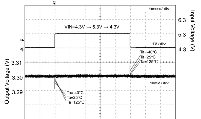
Figure 28. VIN Response
