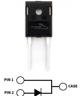
Package Types: TO-247-2 Marking: C4D15120
