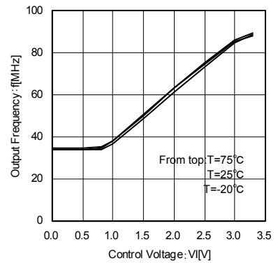
Fig.33 Control Voltage – Output Frequency (VDD=3.3V, Rbias=3.0KΩ)
