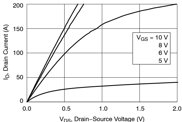
Figure 1. On-Region Characteristics
