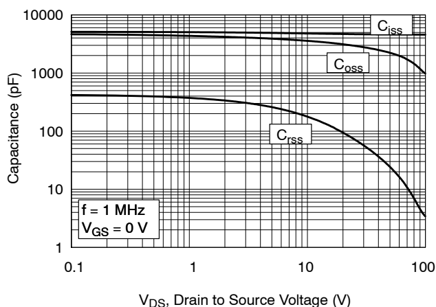
Figure 6. Capacitance Variation
