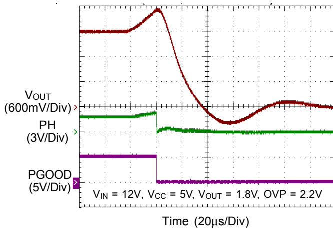
Over-Voltage Protection
