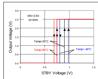
Fig 111. STBY Threshold
