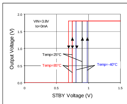
Fig 60. STBY Threshold
