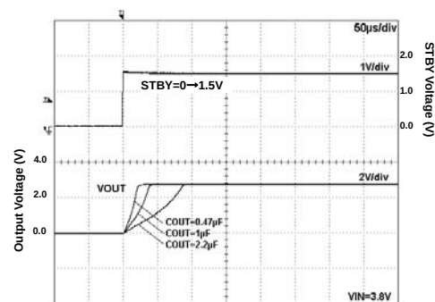
Fig 202. Start Up Time I_{out}=200mA
