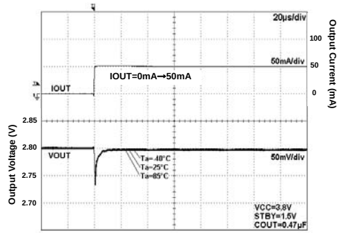
Fig 193. Load Response
