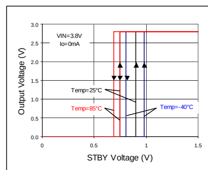
Fig 189. STBY Threshold
