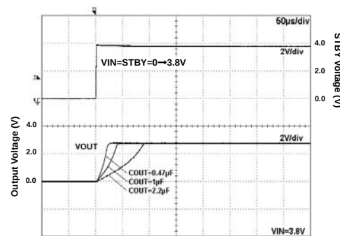
Fig 204. Start Up Time ( V_{IN}=STBY ) I_{out}=200mA
