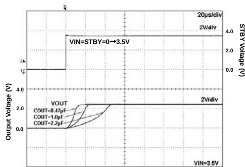
Fig 125. Start Up Time (VIN=STBY) Iout=0mA
