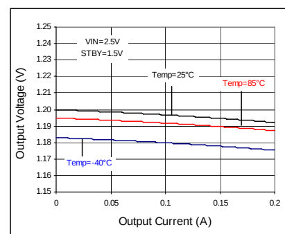
Fig 8. Load Regulation
