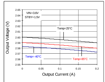
Fig 134. Load Regulation
