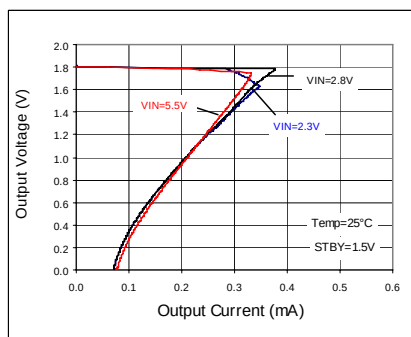
Fig 59. OCP Threshold
