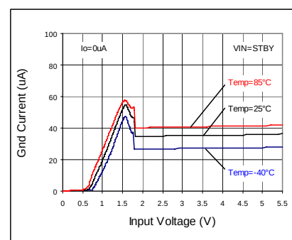
Fig 55. Circuit Current IGND
