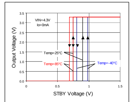
Fig 267. STBY Threshold
