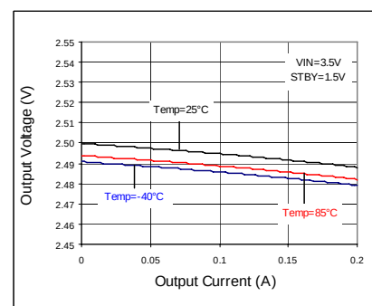
Fig 108. Load Regulation
