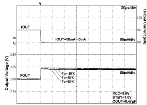
Fig 194. Load Response
