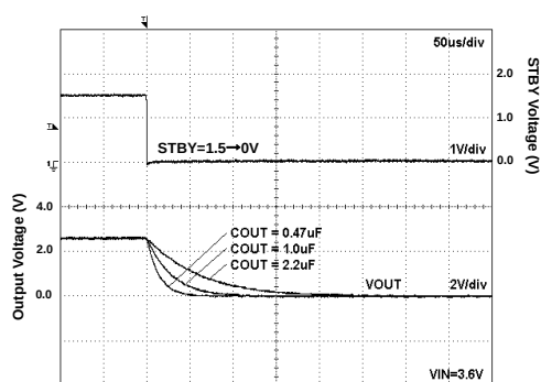
Fig 153. Discharge Time
