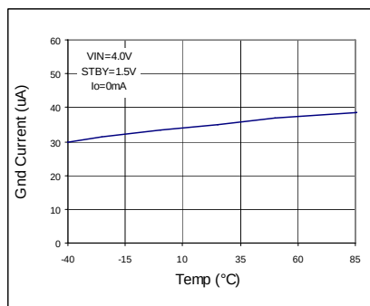
Fig 217. IGND - Temp
