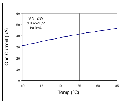
Fig 62. IGND - Temp
