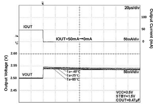
Fig 116. Load Response
