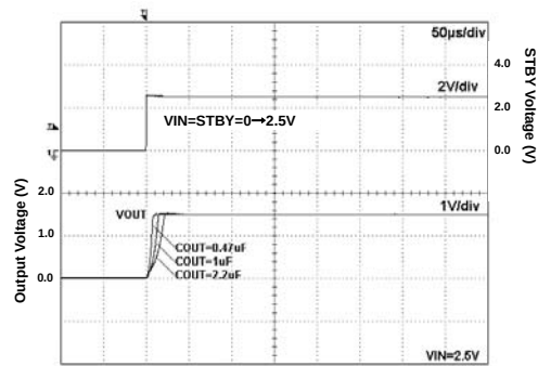
Fig 49. Start Up Time (VIN=STBY) Iout=0mA Iout=0mA
