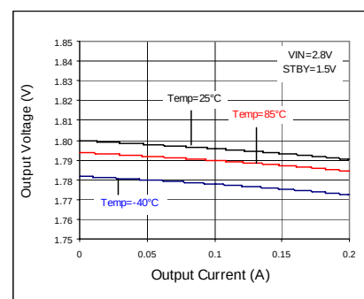
Fig 58. Load Regulation
