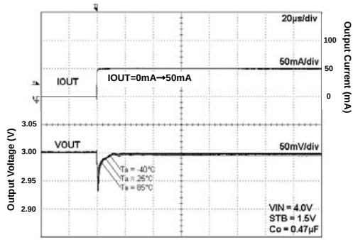
Fig 219. Load Response
