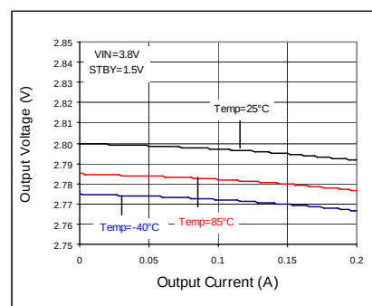
Fig 186. Load Regulation
