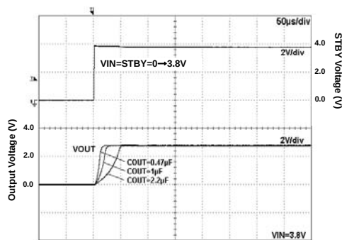
Fig 203. Start Up Time ( V_{IN}=STBY ) I_{out}=0mA I_{out}=0mA
