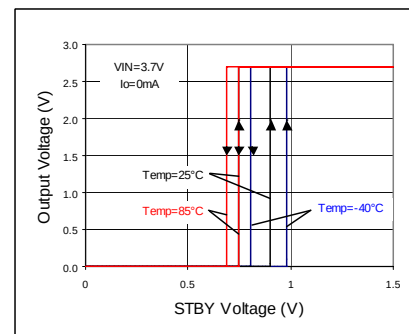
Fig 163. STBY Threshold
