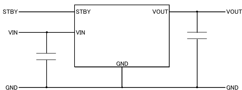
Fig.1 Application Circuit
