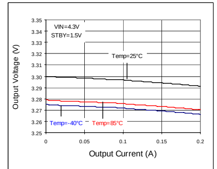
Fig 264. Load Regulation
