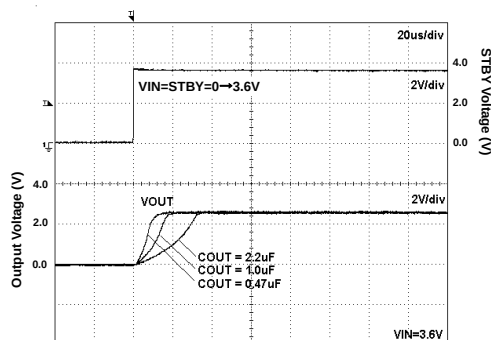
Fig 151. Start Up Time (VIN=STBY) Iout=0mA
