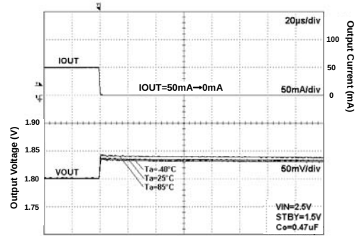
Fig 65. Load Response
