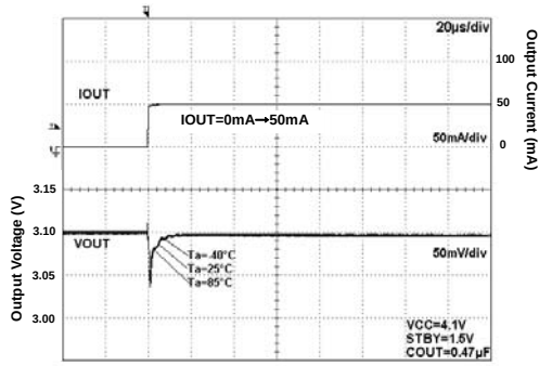
Fig 245. Load Response
