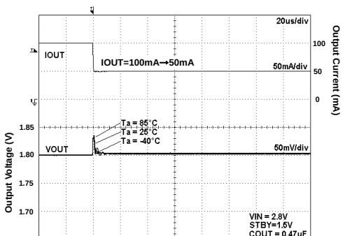
Fig 71. Load Response
