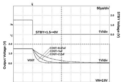
Fig 51. Discharge Time
