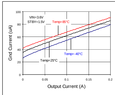
Fig 133. IOUT - IGND
