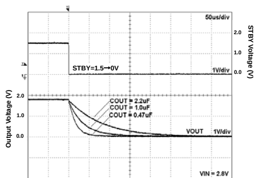
Fig 76. Discharge Time
