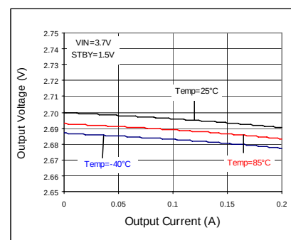
Fig 160. Load Regulation
