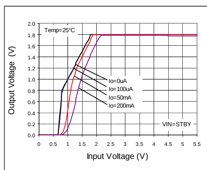
Fig 53. Output Voltage
