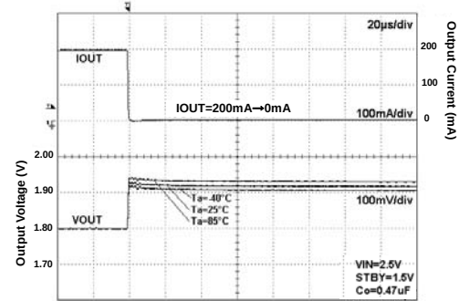
Fig 69. Load Response
