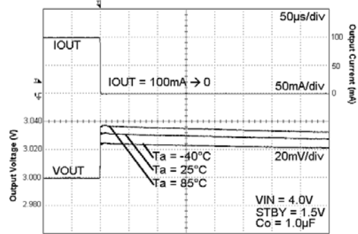
Fig. 137 Load Response
