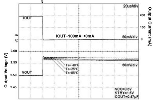
Fig 118. Load Response
