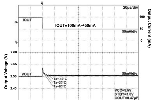
Fig 122. Load Response
