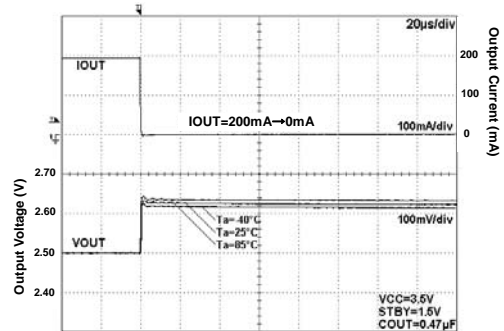
Fig 120. Load Response
