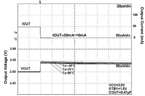
Fig 116. Load Response
