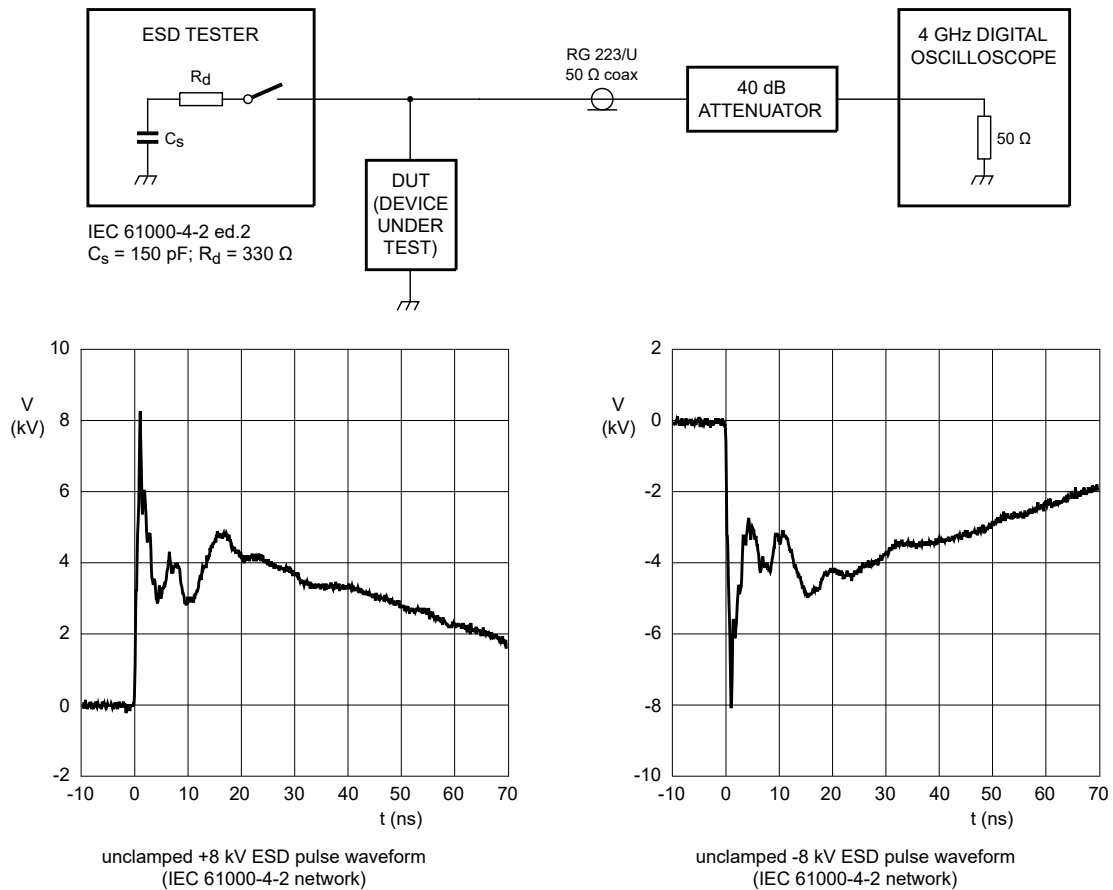
Fig. 10. ESD clamping test setup and waveforms
