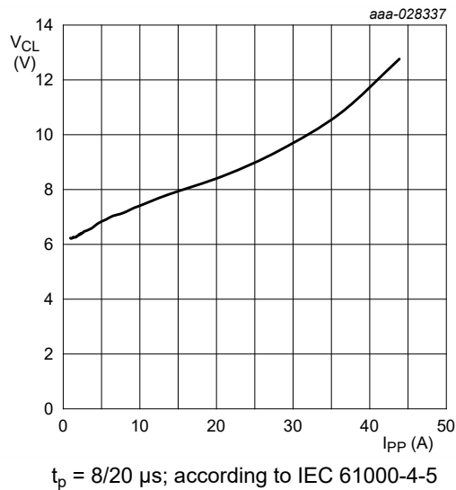
Fig. 7. Positive clamping voltage (8/20 \mu s pulse); typical values
