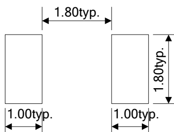
Recommended Pad Layout (mm)
