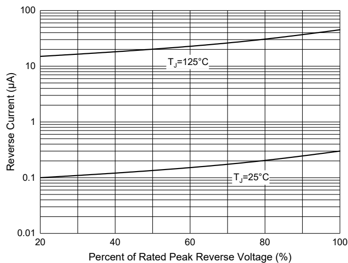
Fig. 4 - Reverse Characteristics
