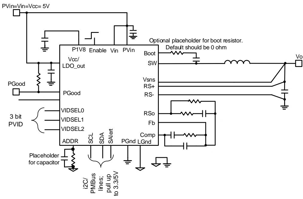
Figure 7: Single 5V application, Vo<2.555V
