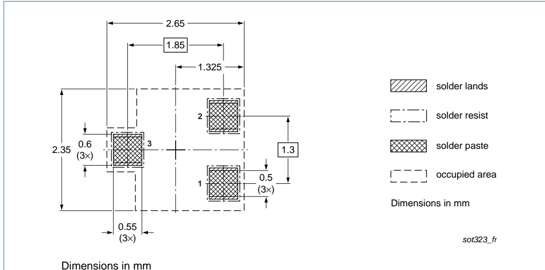
Fig 54. Reflow soldering footprint PDTD1xxxU series (SOT323/SC-70)
