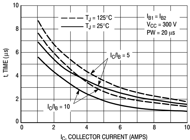
Figure 12. Resistive Switch Time, t_{off}
