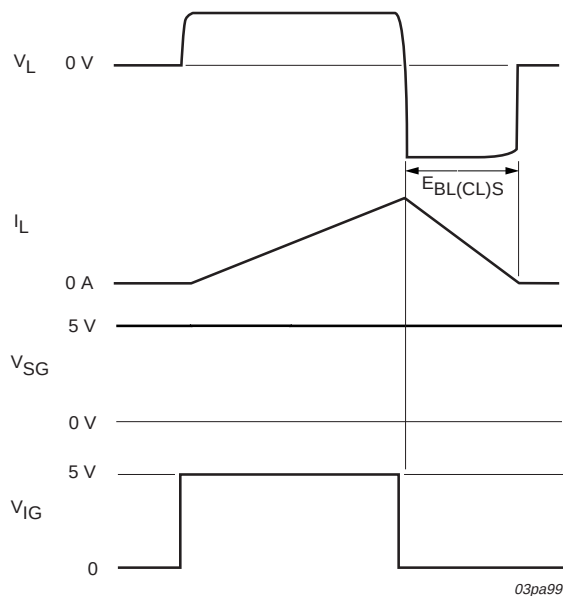
Fig 13. Switching a large inductive load.
