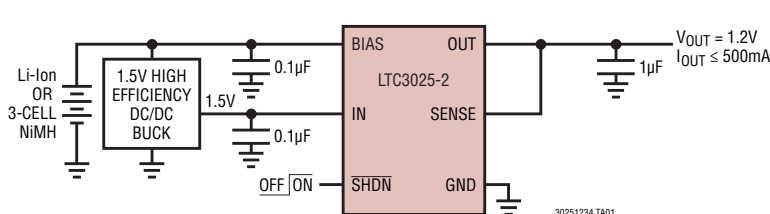
1.2V Output Voltage from 1.5V Input Supply
