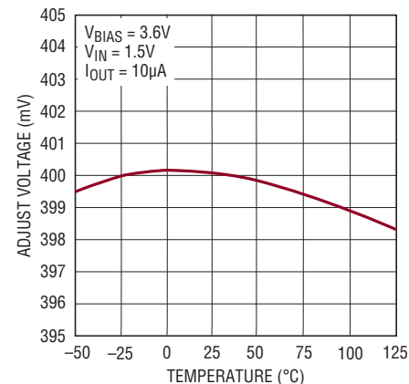
Adjust Voltage vs Temperature
