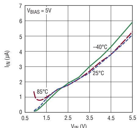
V_{IN} Shutdown Current
