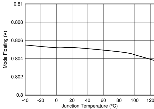
Figure 7-15. Mode Floating vs Temperature
