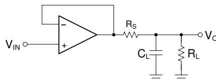
Figure 8-1. OPA810 Driving Capacitive Load
