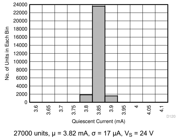
Figure 7-57. Quiescent Current Distribution
