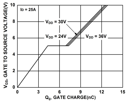
Figure 16. Gate Charge vs. Gate to Source Voltage
