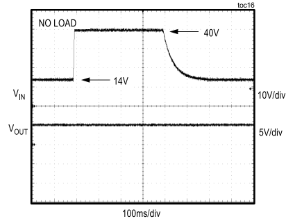
LOAD-DUMP TEST
