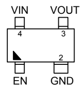
SC-82 (SSOT-24)
