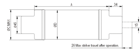
SJ Fuses
