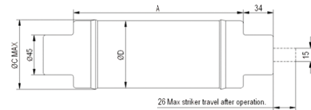
SJ Fuses
