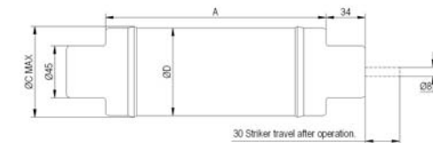
EJ Fuses
