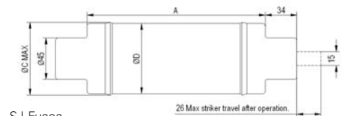
SJ Fuses
