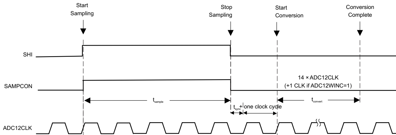
Figure 34-3. Extended Sample Mode Without Internal Reference in 12-Bit Mode
