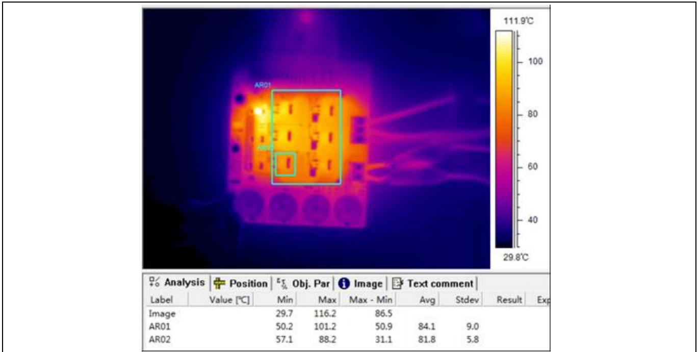
Figure 20 Thermal test
