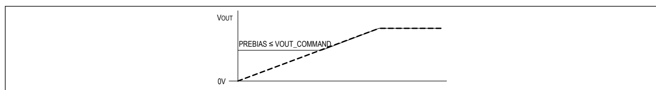
Figure 4. Prebias Startup
