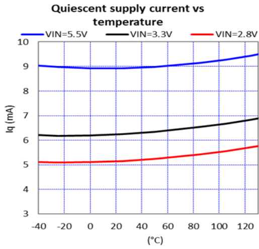
Figure 10. Quiescent Current vs. Temperature (EN = High, V_{OUT} = 1.8\text{ V} , No Load)
