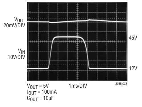
Transient Response (Load Dump)
