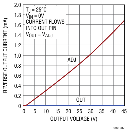
Figure 7. LT3060 Reverse Output Current
