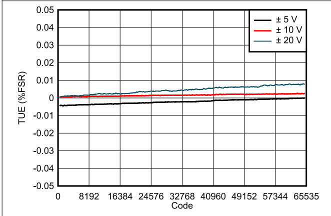
Figure 7-7. DAC81402 TUE vs Digital Input Code (Bipolar Outputs)
