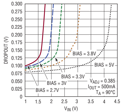
V IN to V OUT Dropout Voltage vs V IN (90°C) LTC3025-1
