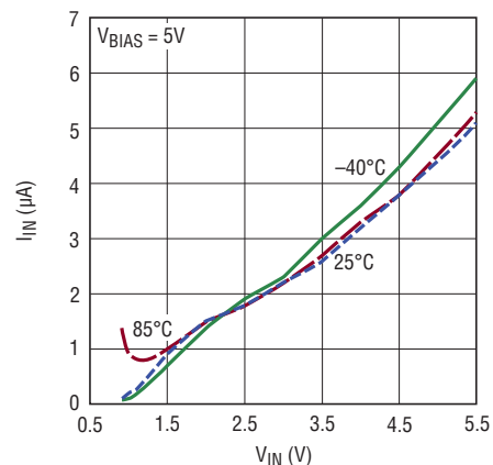
I_{IN} Shutdown Current
