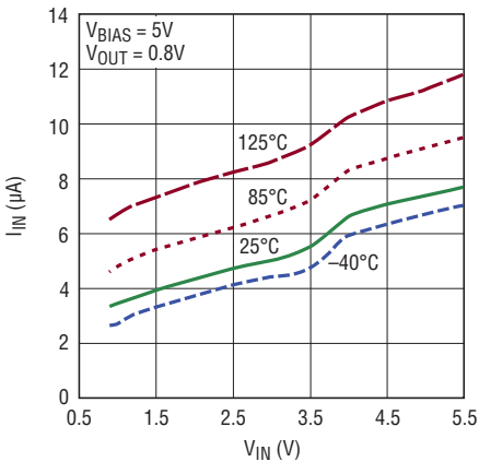
I_{IN} No Load Operating Current
