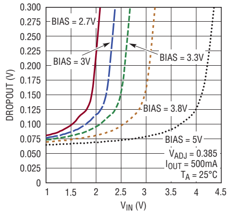
V IN to V OUT Dropout Voltage vs V IN (25°C) LTC3025-1
