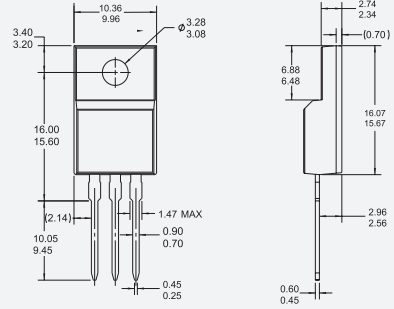
TO-220 [KF]
