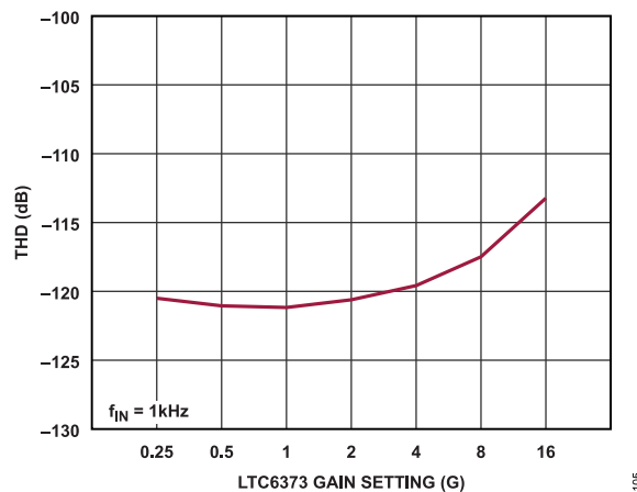
Figure 104. THD for LTC6373 + ADA4945-1 + AD7768-1 Signal Chain
