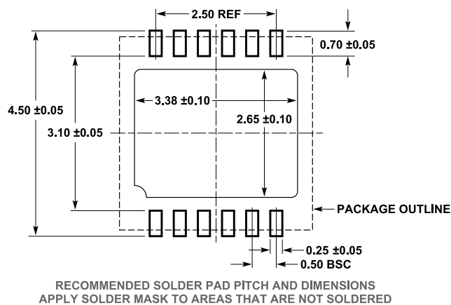
Figure 106. 12-Lead 4 mm \times 4 mm DFN (05-08-1791)
