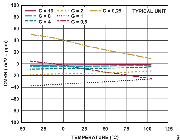
Figure 23. CMRR vs. Temperature
