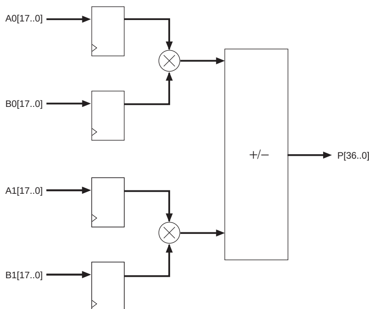
Figure 5–2. Basic Two-Multiplier Adder Building Block
