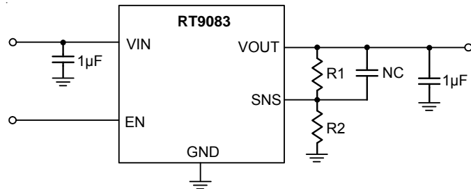
Figure 3. Adjustable Output Voltage Application Circuit
