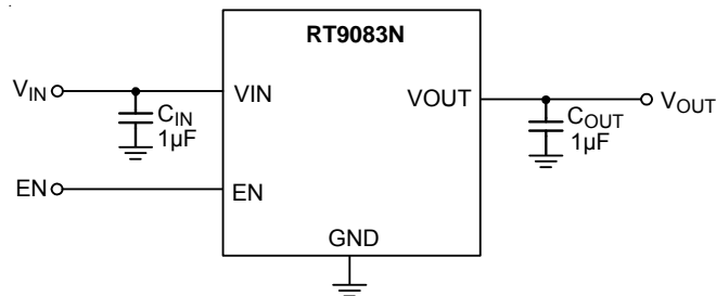
Figure 2. Application without Sense Function
