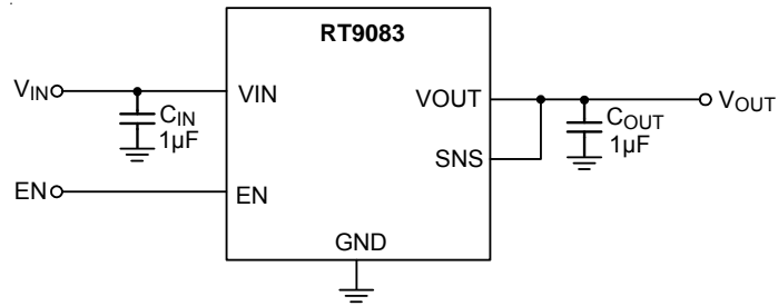
Figure 1. Application with Sense Function
