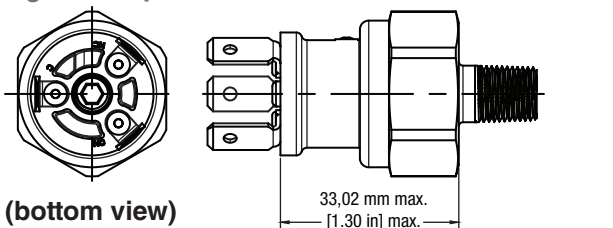
Figure 25. Spade terminal
