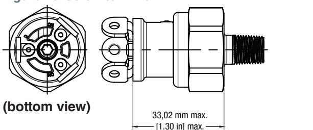
Figure 26. Screw terminal
