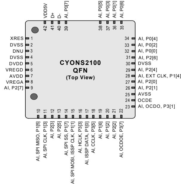
Figure 3. Pin Diagram
