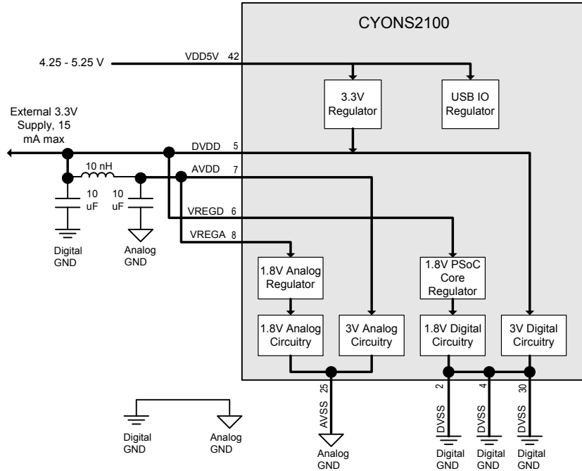
Figure 6. Power Connections
