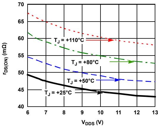
FIGURE 7. LOW-SIDE r_{DS(on)} vs V_{DDS} WITH T_J
