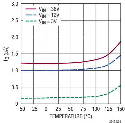
Combined PVIN/VIN Shutdown Current
