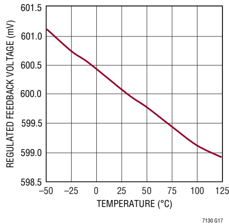
Regulated Feedback Voltage vs Temperature
