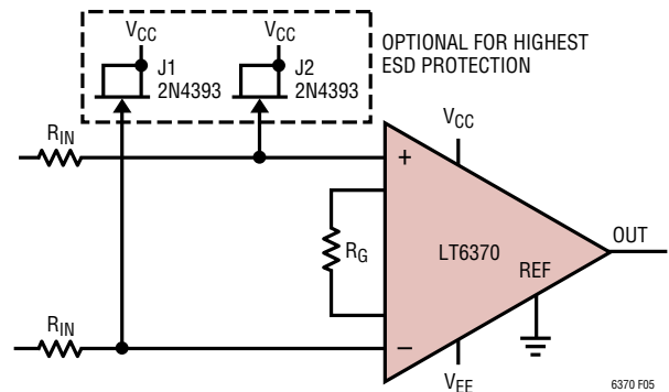
Figure 9. Input Protection
