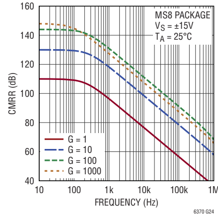
CMRR vs Frequency, RTI MS8 Package
