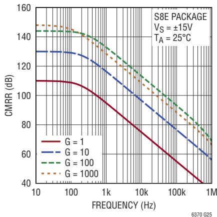
CMRR vs Frequency, RTI S8E Package
