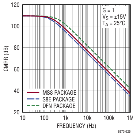
CMRR vs Frequency, RTI
