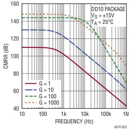
CMRR vs Frequency, RTI DD10 Package
