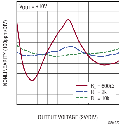
Gain Nonlinearity (G = 1000)
