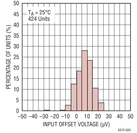
Distribution of Input Offset Voltage, DD10 Package
