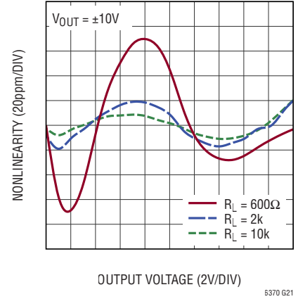
Gain Nonlinearity (G = 100)
