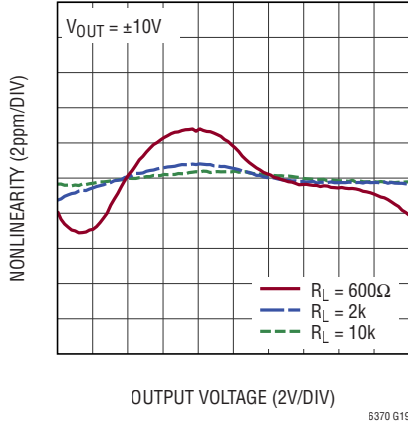
Gain Nonlinearity (G = 1)
