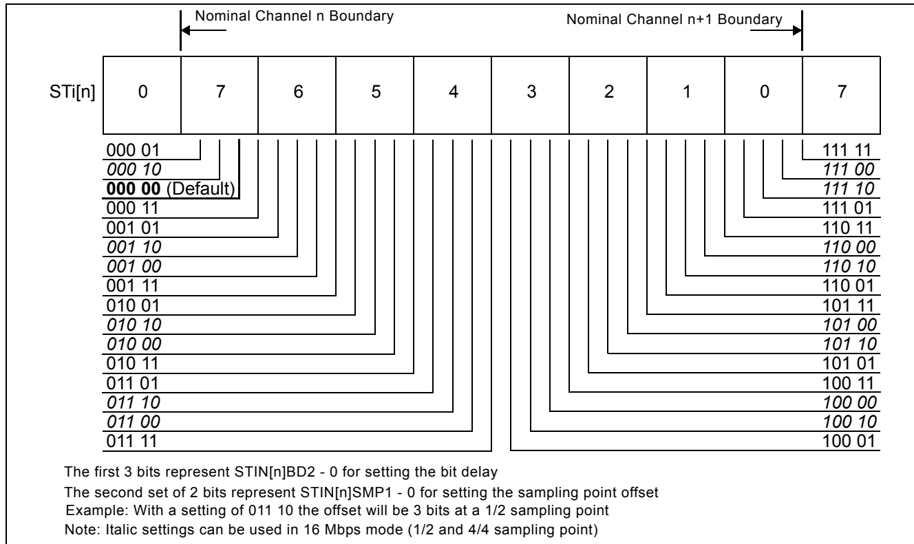
Figure 13 - Input Bit Delay and Factional Sampling Point
