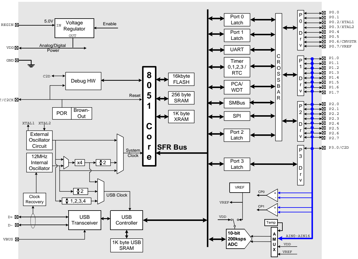
Figure 1.1. C8051F320 Block Diagram
