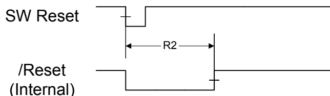
Figure 25-11. Software Reset Timing
