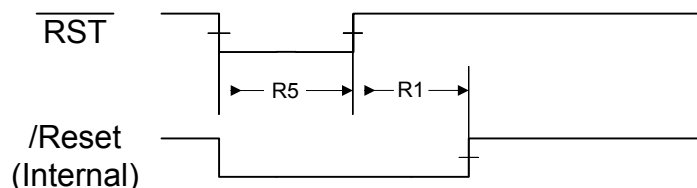
Figure 25-10. External Reset Timing ( \overline{\text{RST}} )
