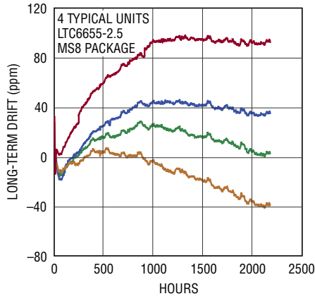
Figure 10a. Long-Term Drift MS8
